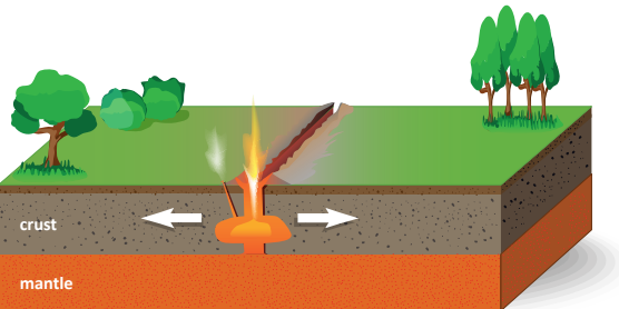
Divergent plate boundary
