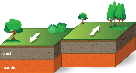
Transform plate boundary
