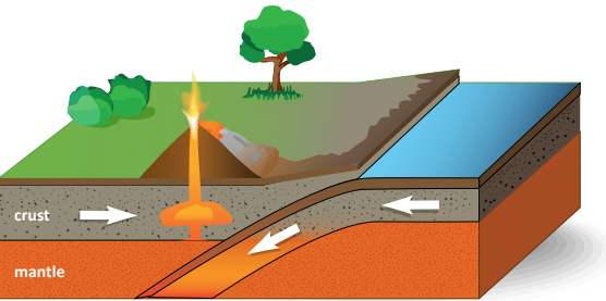
Convergent plate boundary
